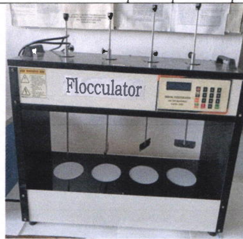
Digital Flocculator
