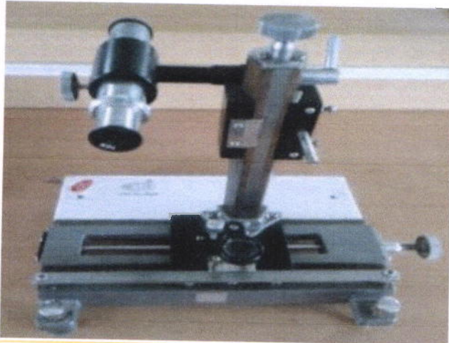
Travelling Microscope
