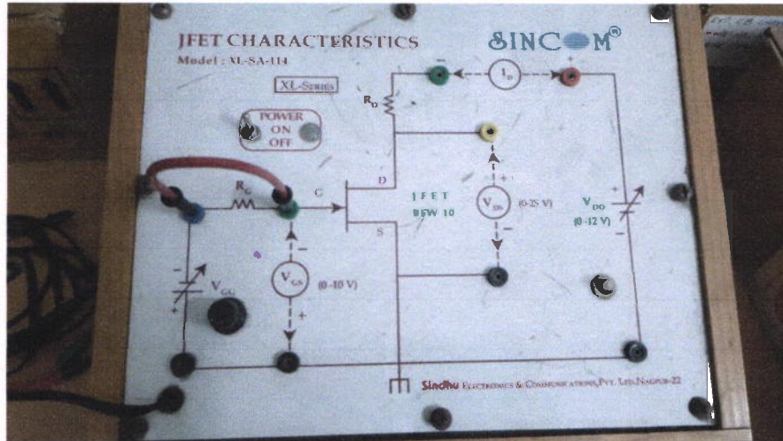
JFET CHARACTERISTICS
